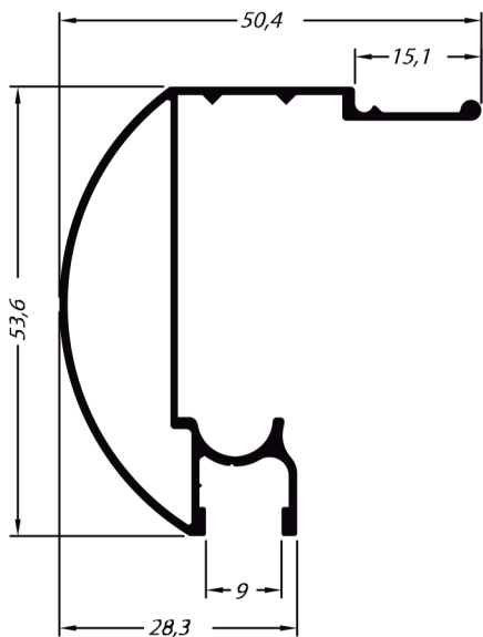
2910 BOX 3,200 kg/6,10m
